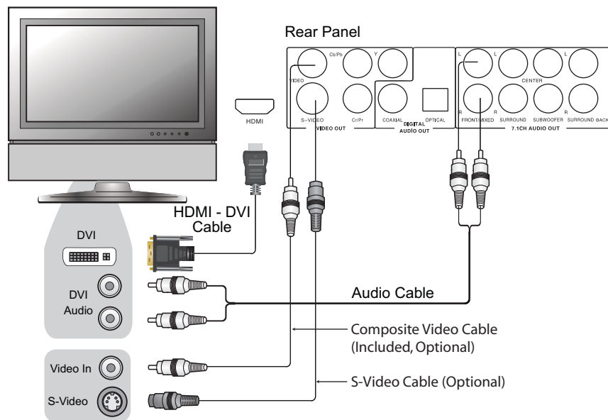
Method 2 – DVI Connection to TV
